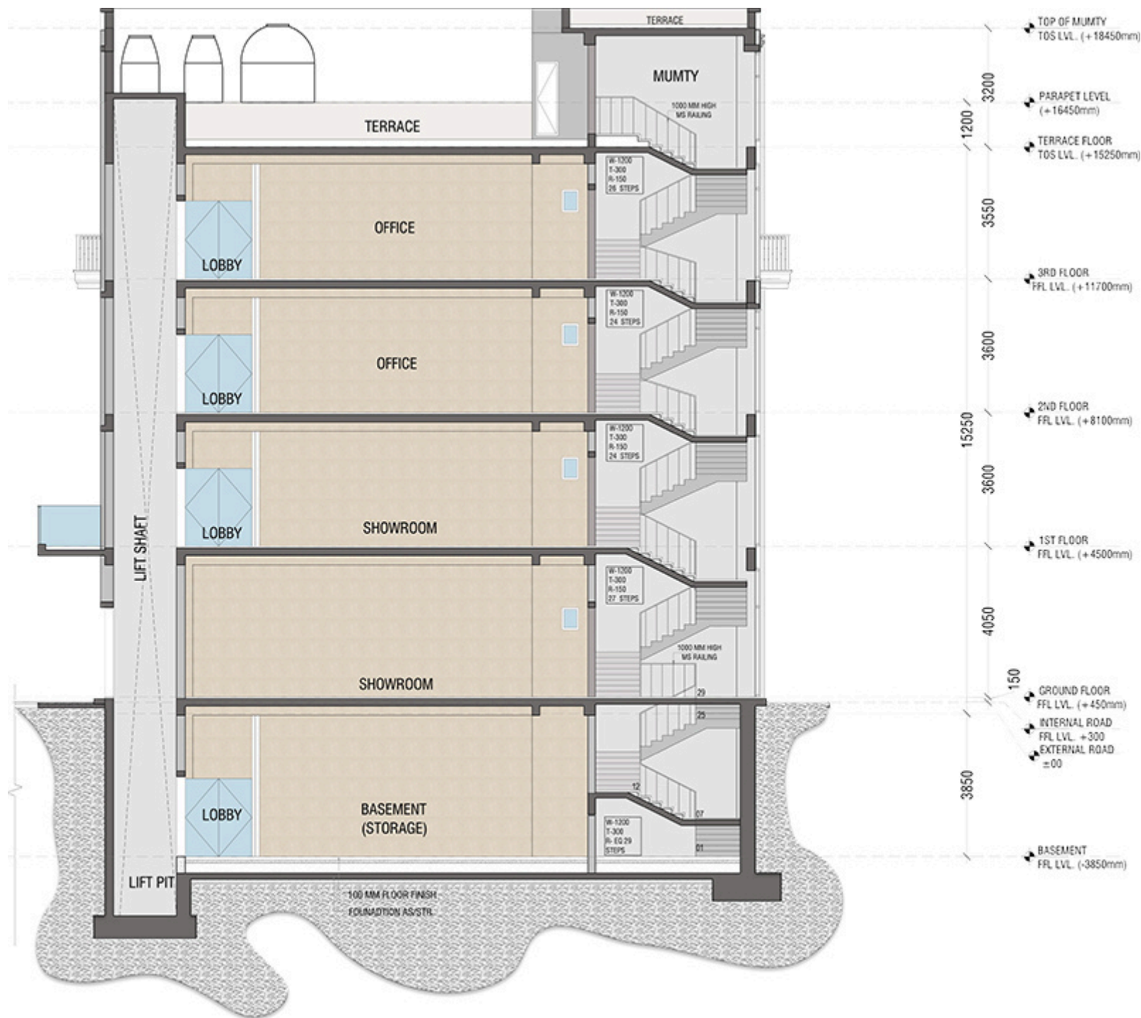
SECTION AA-TYPICAL
